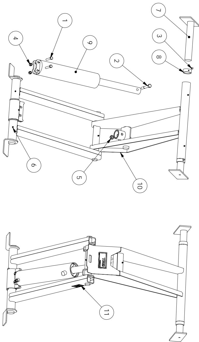
MODEL TB-10 OR TH-410 HOIST PARTS LIST EFF. 05/24/2006
