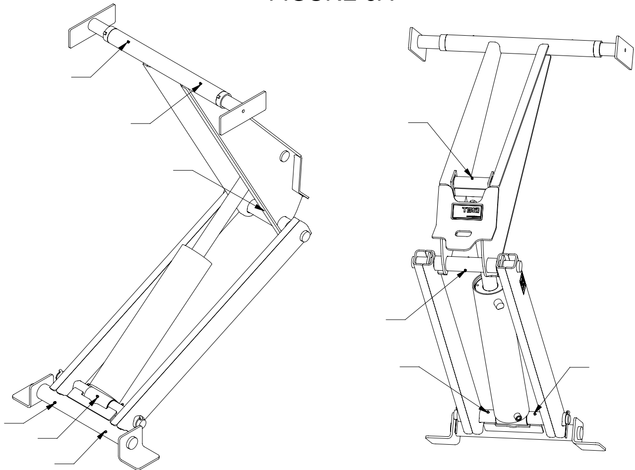
GREASE FITTING LOCATIONS: TB-14 or TH-544
