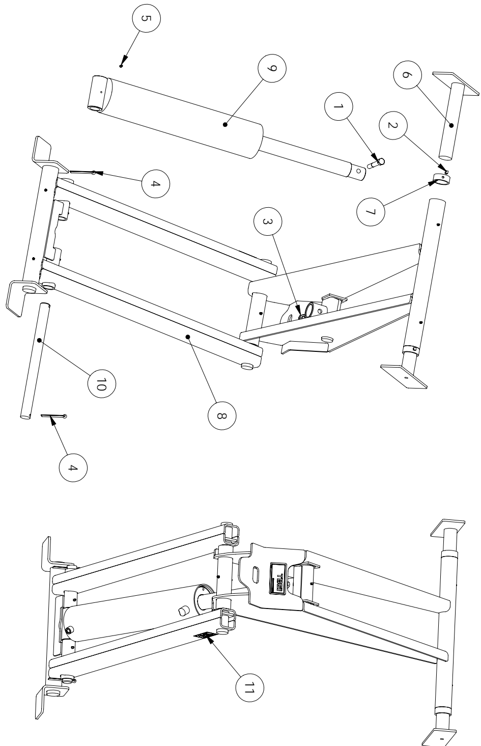
MODEL TB-14 OR TH-544 HOIST PARTS LIST EFF. 05/24/2006
